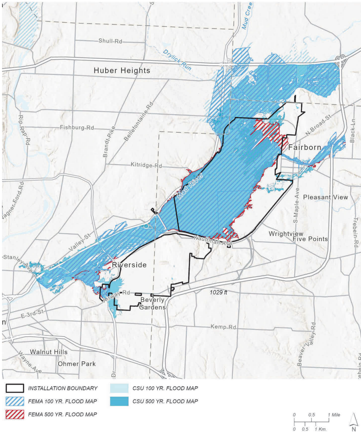
Figure 3 Differences in 100-year and 500-year floodplain area projection between FEMA and CEMML/CSU Engineering for WPAFB.
